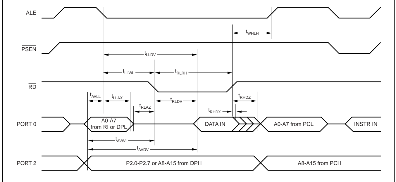
FIGURE B. External Data Memory Read Cycle
