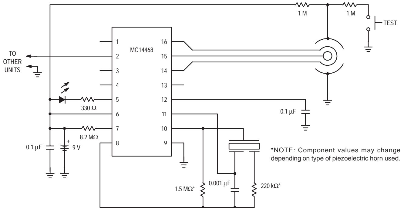
Figure 5. Typical Application as Ionization Smoke Detector
